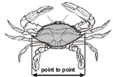
Blue Crab (point to point)
